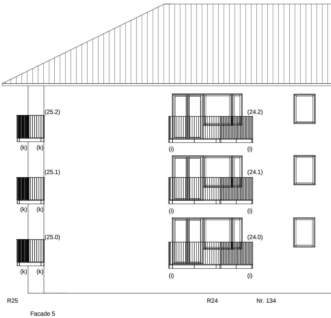
Facade 5
